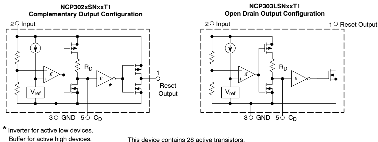
Figure 1. Representative Block Diagrams
