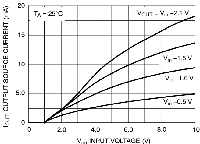
Figure 15. NCP302L Series 0.9 V Reset Output Source Current vs. Input Voltage
