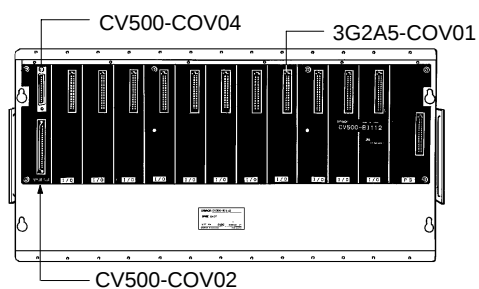
Expansion I/O Rack
