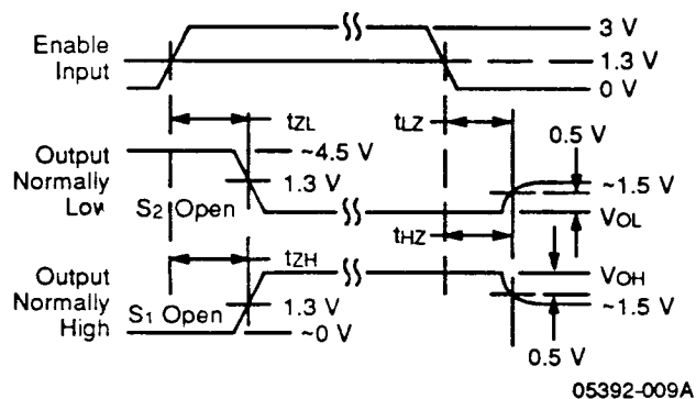
Enable and Disable Times (Notes 2 and 3)
