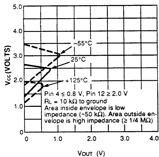
V_{OUT} Versus V_{CC}
