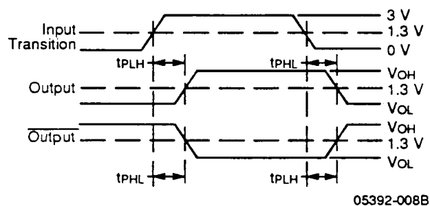
Propagation Delay (Notes 1 and 3)
