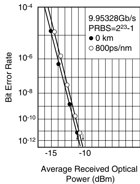
Fig. 6 Transmission Characteristics
