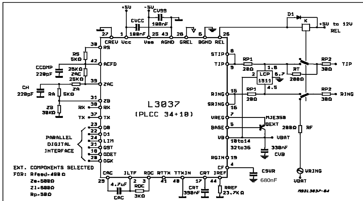
Figure 4: Typical Application circuit with minimum components count (No Rev. polarity NoTTX/No zero crossing sync/no PTC mismatch compensation).
