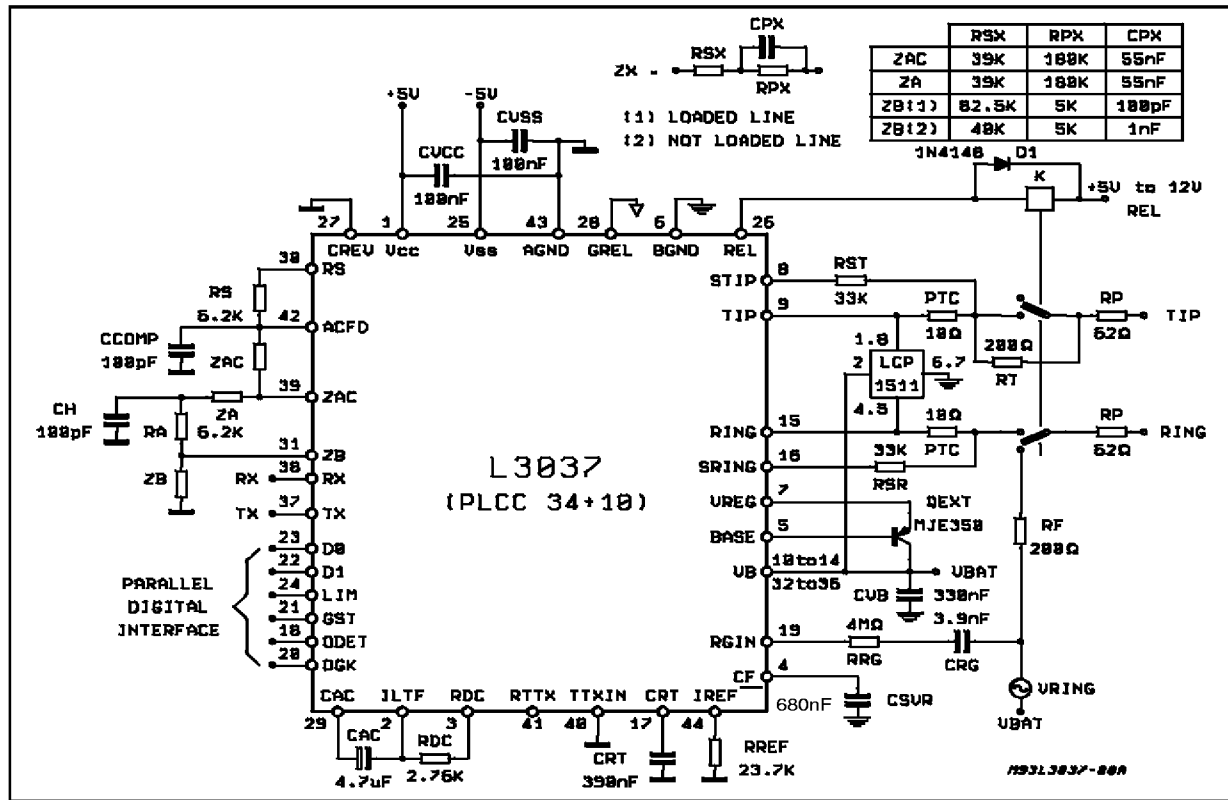
Figure 5: Typical Application Circuit for U.S. Application.
