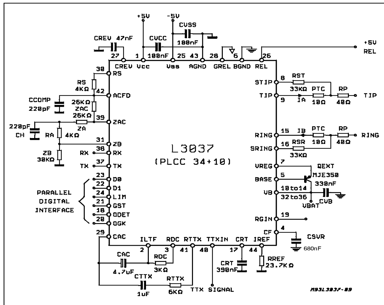
Figure 6: Test Circuit
