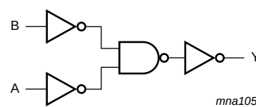
Fig 3. Logic diagram
