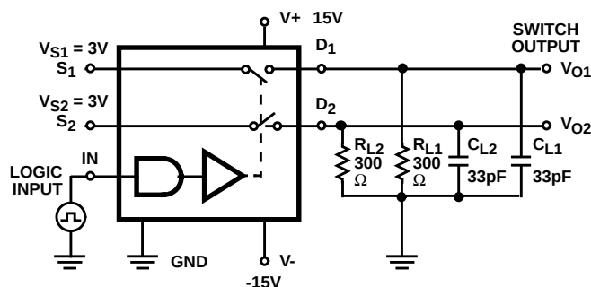
FIGURE 2. BREAK-BEFORE MAKE TEST CIRCUIT AND MEASUREMENT POINTS (DG301A, DG303A)
