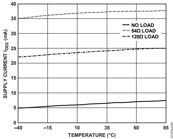
Figure 4. ADM2487E I_{DD2} Supply Current vs. Temperature (See Figure 25) (Data Rate = 500 kbps, V_{DD1} = 5 V, V_{DD2} = 3.3 V, DE = 1 V, RE = 0 V)
