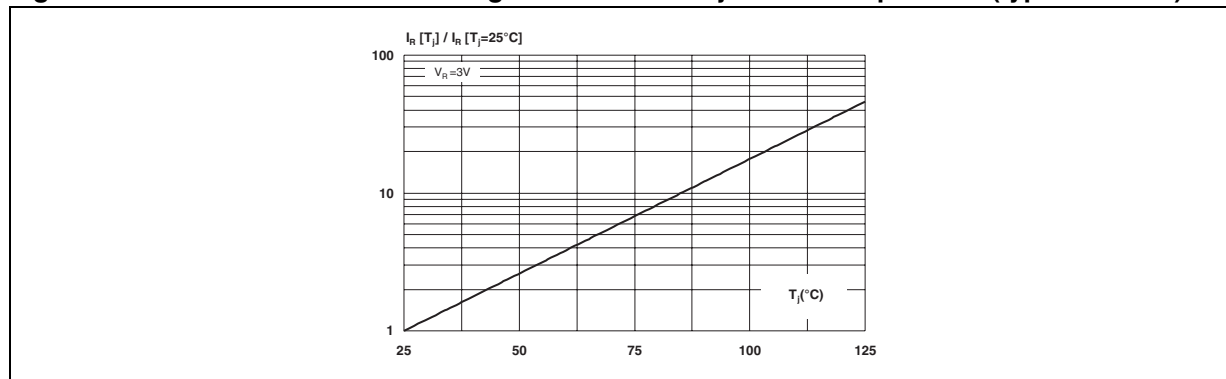
Figure 7. Relative variation of leakage current versus junction temperature (typical values)
