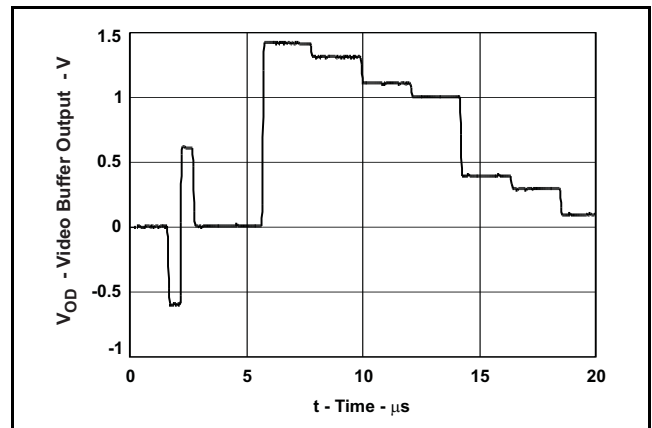
Figure 50. Video Buffer Differential Output Signal
