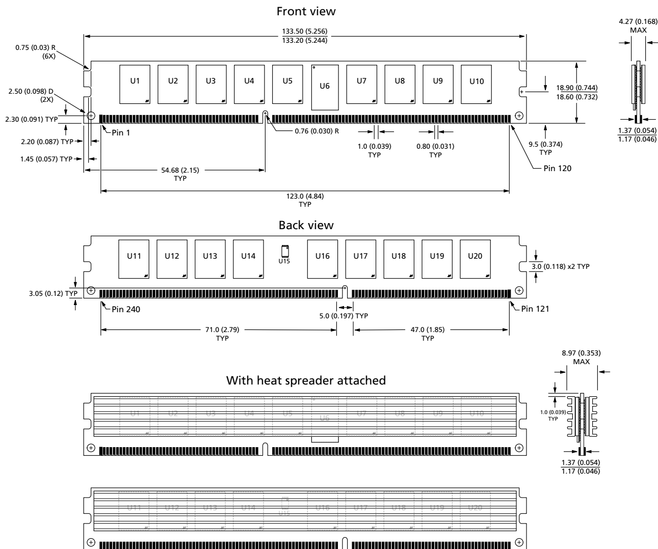
Figure 3: 240-Pin DDR3 RDIMM
