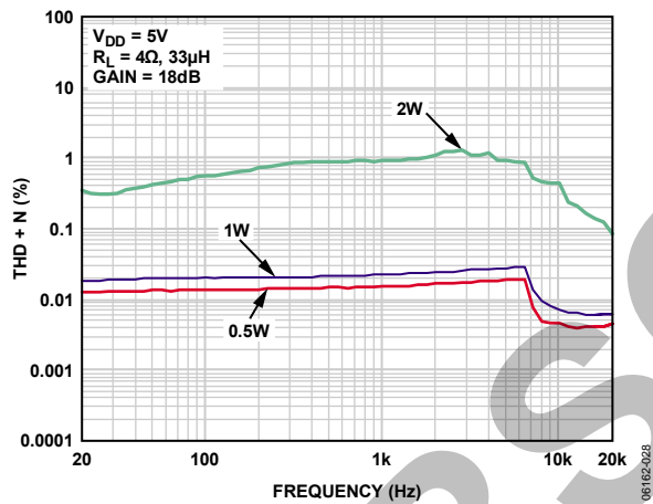
Figure 16. THD + N vs. Frequency, V_{DD} = 5\text{ V} , R_L = 4\ \Omega , A_v = 18\text{ dB}
