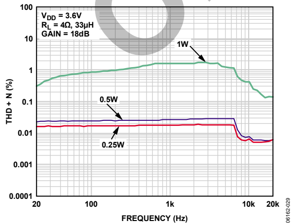
Figure 17. THD + N vs. Frequency, V_{DD} = 3.6\text{ V} , R_L = 4\ \Omega , A_v = 18\text{ dB}
