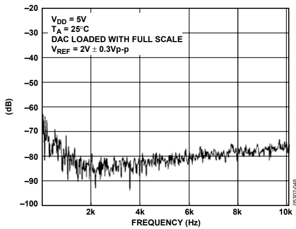
Figure 47. Total Harmonic Distortion
