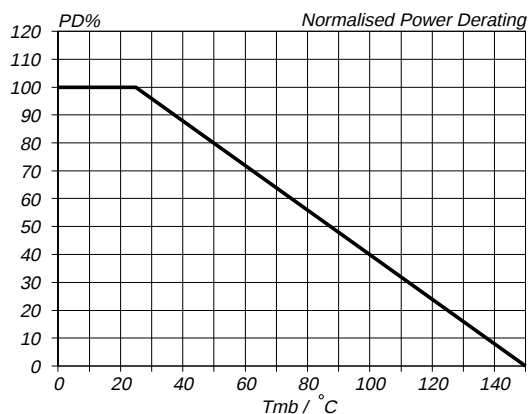
Fig.12. Normalised power dissipation. PD\% = 100 \cdot P_D / P_{D 25^\circ\text{C}} = f(T_{\text{mb}})
