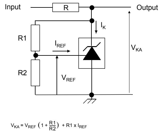
Figure 7. Test circuit for V_{KA} > V_{REF}
