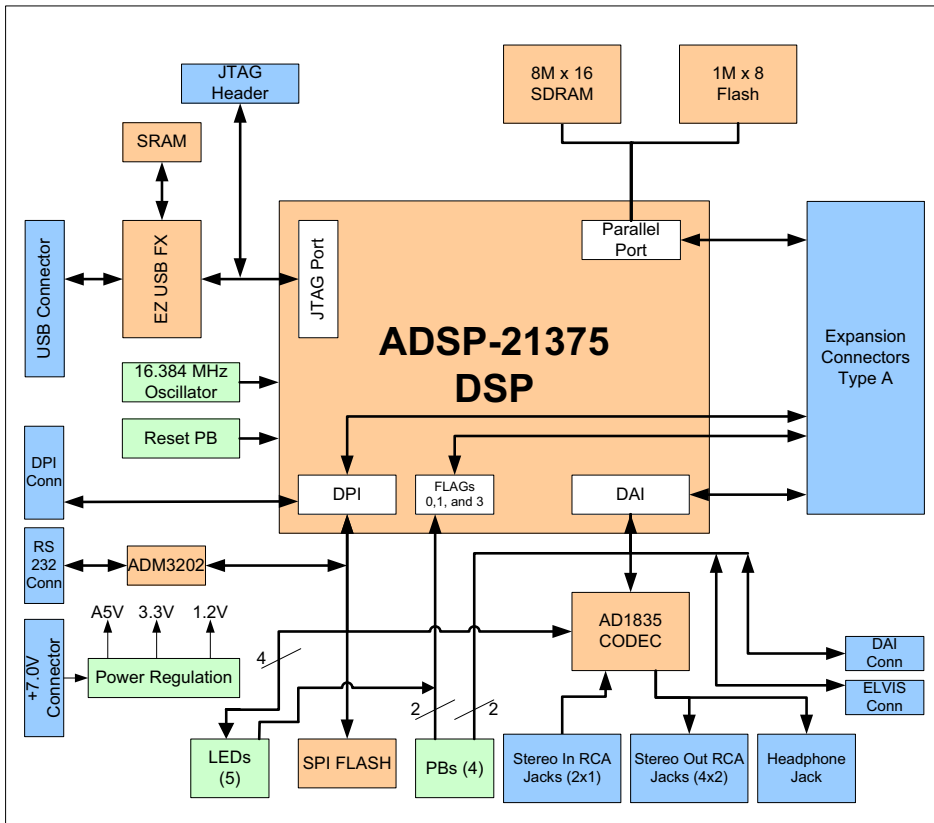
Figure 2-1. System Architecture Block Diagram
