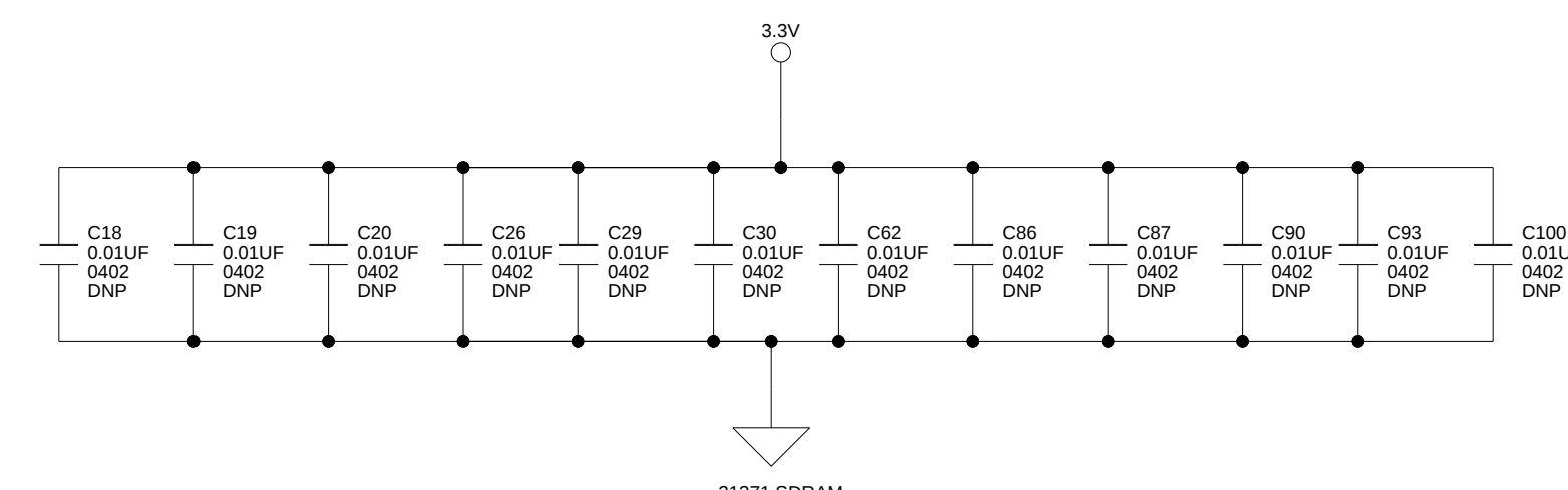
21371 SDRAM
