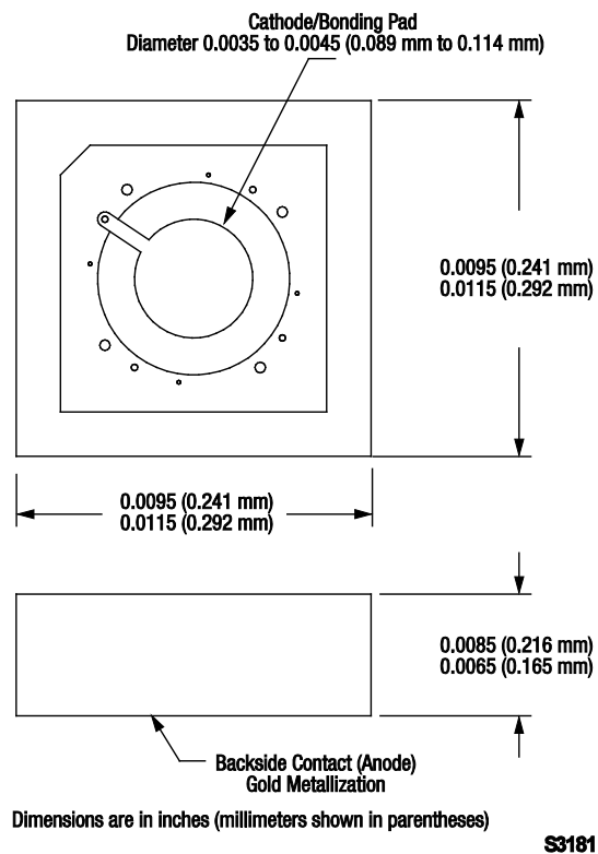
Figure 12. 571-006 Package Dimensions
