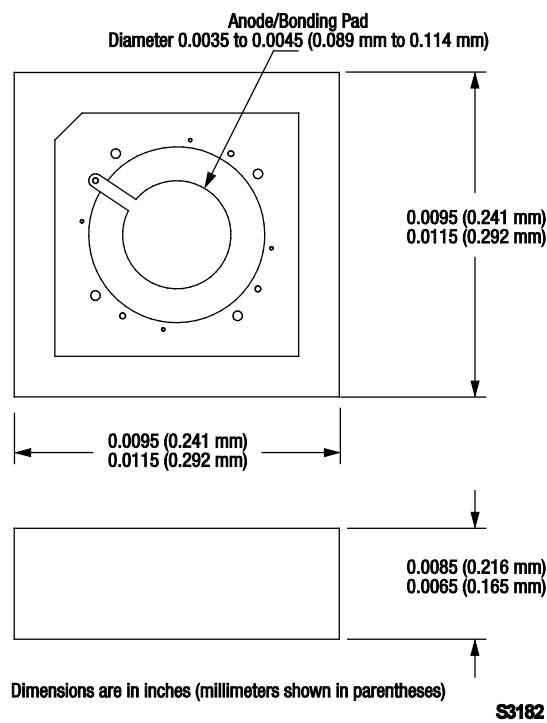
Figure 13. 571-011 Package Dimensions
