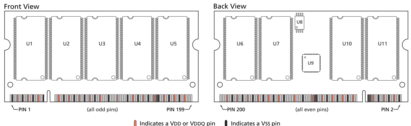
Figure 1: Module Layout
