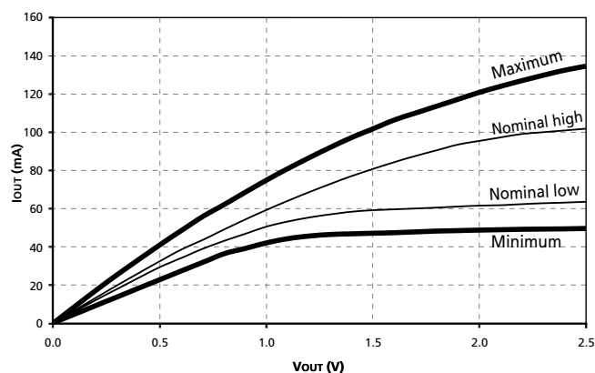
Figure 8: Pull-Up Characteristics
