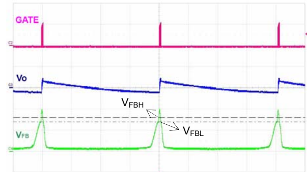
Figure 29. Burst-Mode Operation
