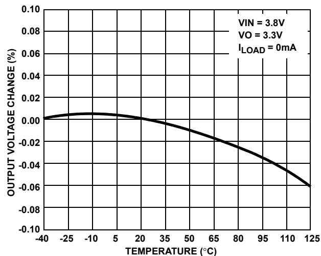
FIGURE 4. OUTPUT VOLTAGE CHANGE vs TEMPERATURE
