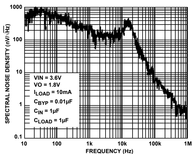
FIGURE 19. SPECTRAL NOISE DENSITY vs FREQUENCY
