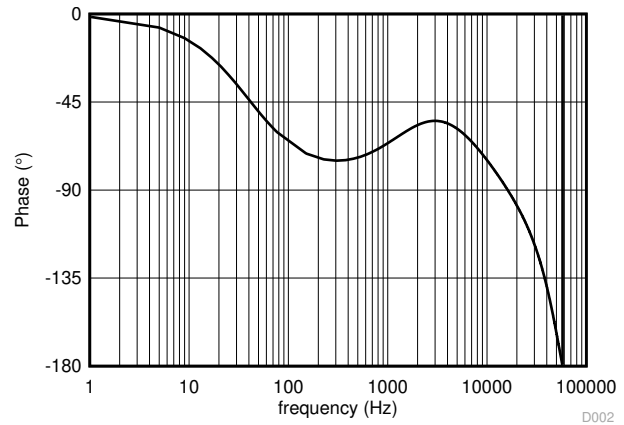
Figure 8-5. Converter Open-Loop Bode Plot - Phase
