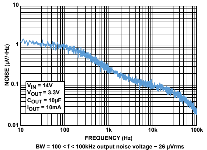
FIGURE 12. OUTPUT NOISE SPECTRAL DENSITY, I_{OUT} = 10mA
