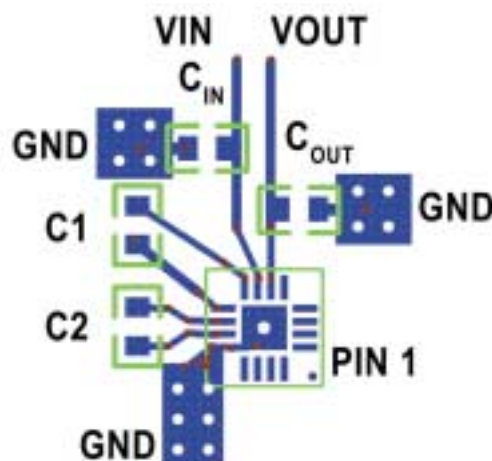
Figure 2: PCB Layout
