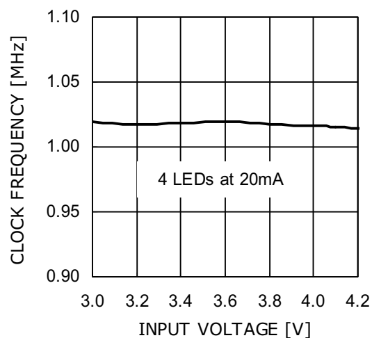
Oscillator Frequency vs. Input Voltage
