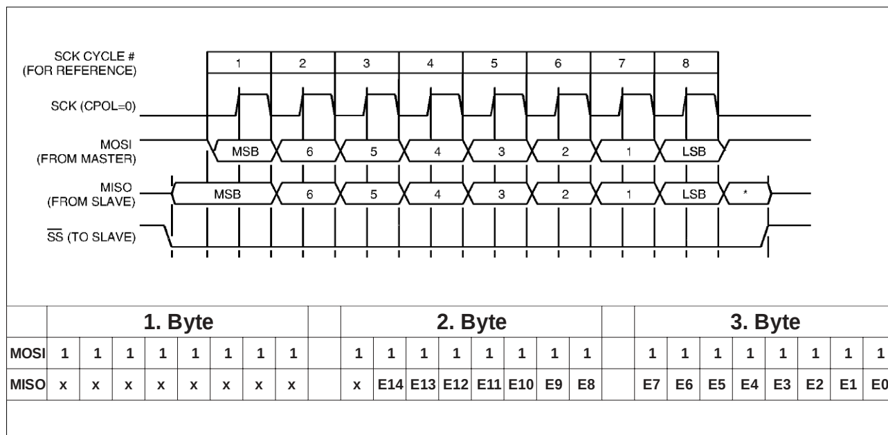
FIGURE I: SPI-BUS Protocol
