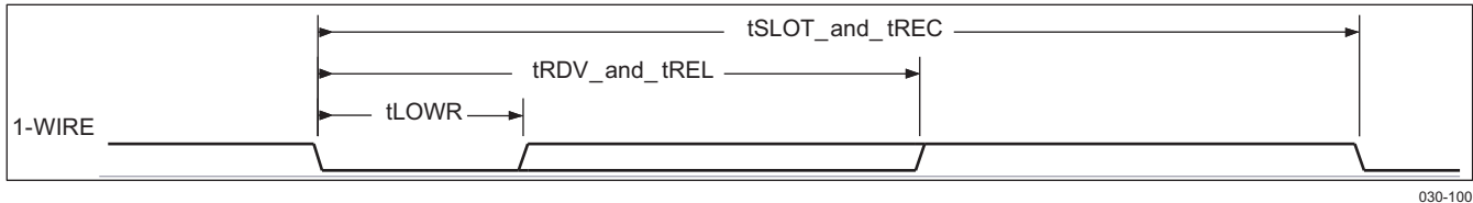
Figure 6-60. 1-Wire Read Bit Timing (Data)
