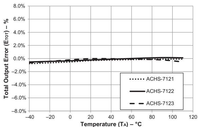
Figure 4: Total Output Error at I_{P\text{MAX}} vs. Temperature
