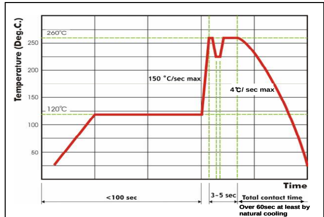
Fig. 11 Recommended wave soldering profile for SMT process with SnAgCu series solder.
