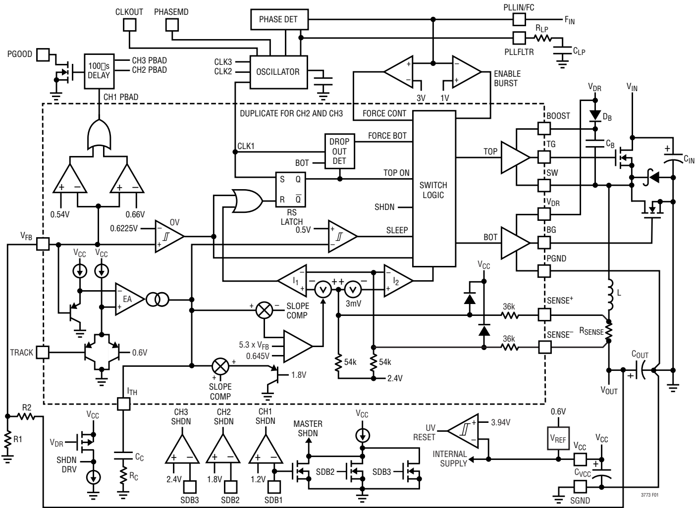
Figure 1. Functional Diagram
