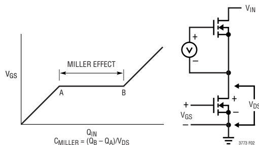
Figure 2. MOSFET Miller Capacitance
