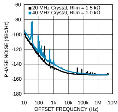
Figure 20. HCSL Phase Noise @ 100 MHz
