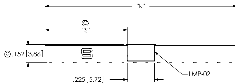
FIG 3 (-P: PICK AND PLACE PAD) AVAILABLE ON POSITIONS 03 THRU 50
