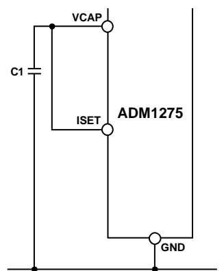
Figure 52. Fixed 20 mV Current Sense Limit
