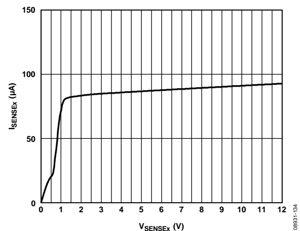
Figure 34. SENSE+/SENSE- Input Current ( I_{SENSEx} ) vs. Voltage ( V_{SENSEx} )
