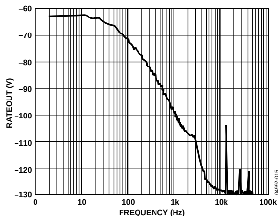
Figure 16. Noise Spectral Density at RATEOUT – BW = 4Hz
