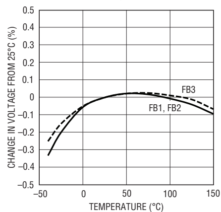
Feedback Voltages
