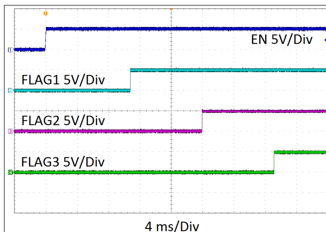
Figure 19. Power-Up Sequence, C_{ADJ} = 10 nF
