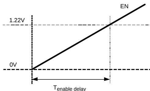
Figure 14. Enable Delay Timing
