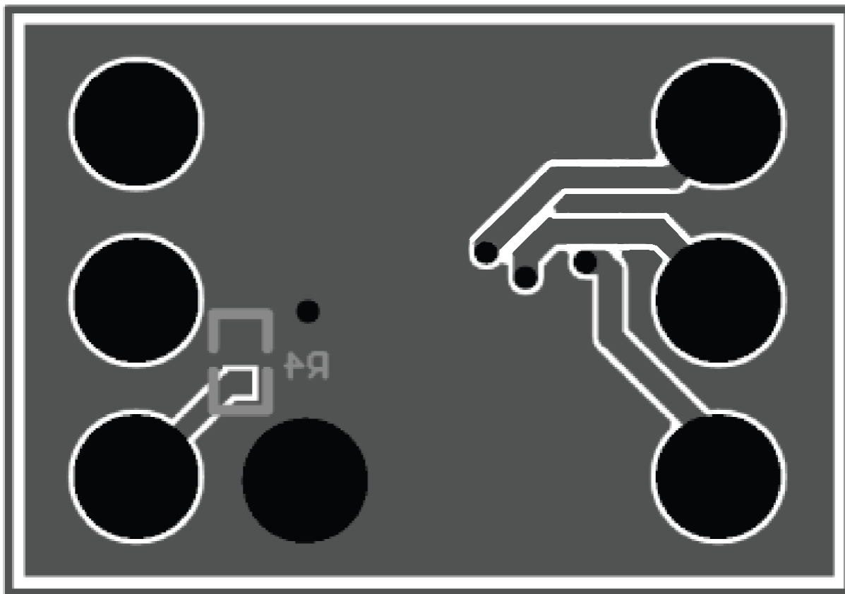
Figure 25. LM3881 Bottom
