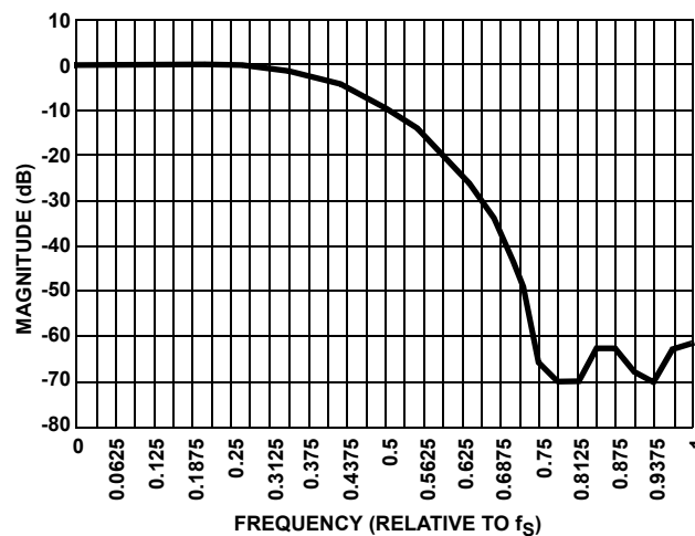
FIGURE 14. POLYPHASE RESAMPLER FILTER PASS BAND FREQUENCY RESPONSE
