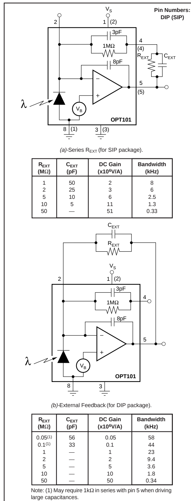
FIGURE 4. Changing Responsivity with External Resistor.
