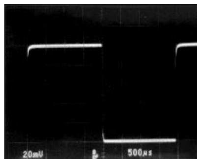
SMALL SIGNAL RESPONSE ( C_{\text{LOAD}} = 10,000\text{ pF} ) (Pin 3 = -15V)
