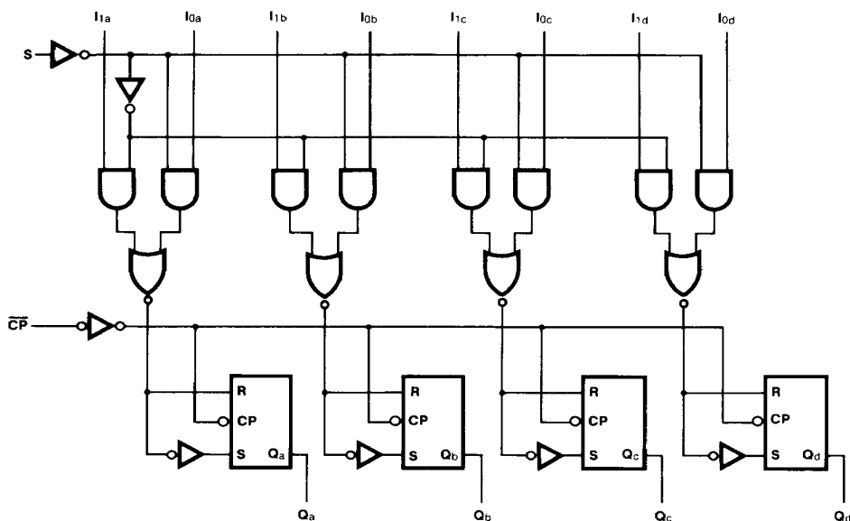
LOGIC DIAGRAM
