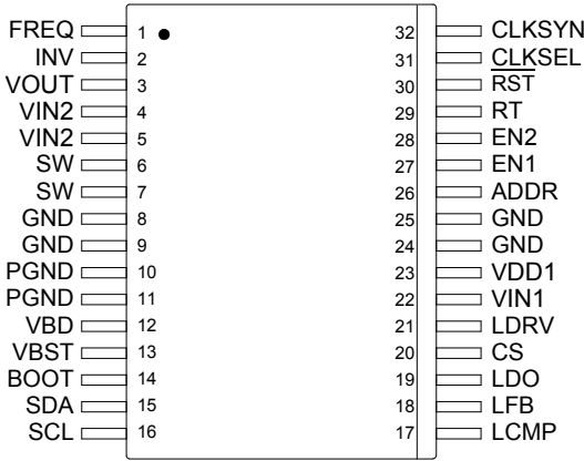
Figure 3. Pin Connections
