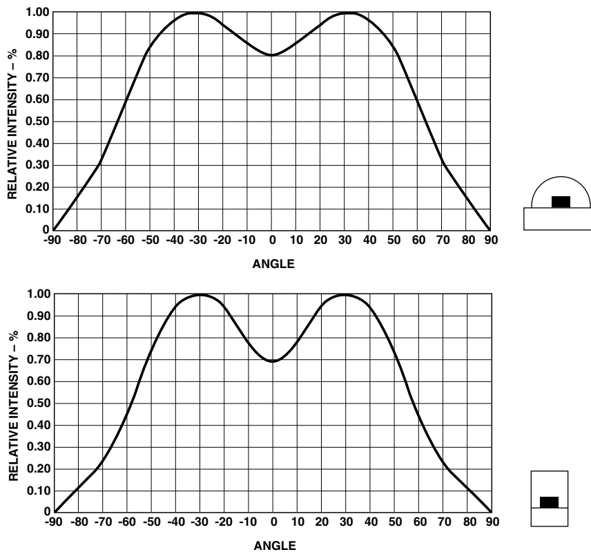
Figure 5. Relative intensity vs. angle for HSMx-C110.
