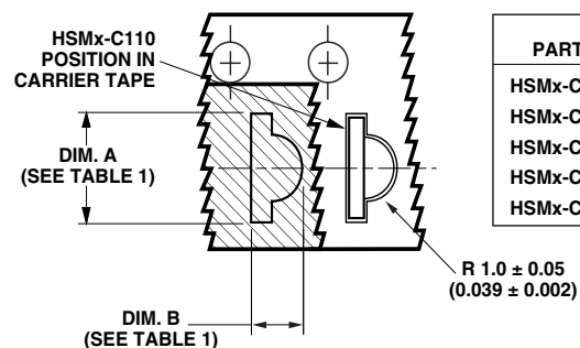
Figure 15. Tape dimensions.
