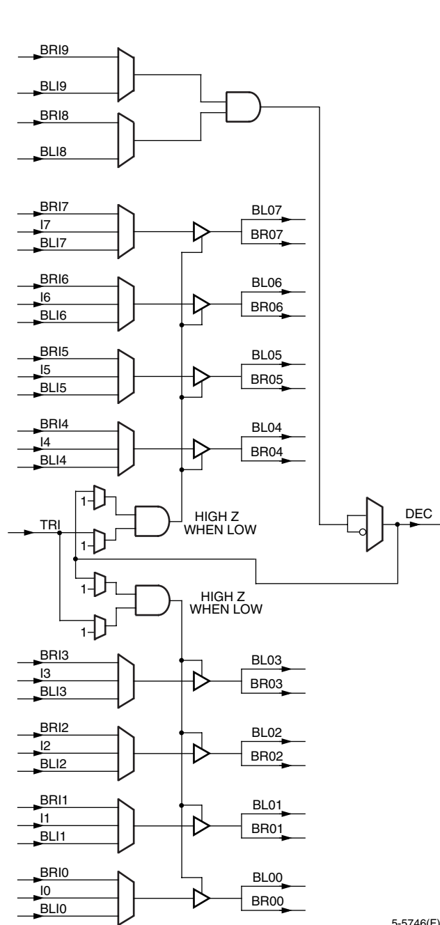
Figure 13. Buffer-Buffer-Decoder Mode
