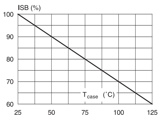
Figure 9: Secondary Breakdown Temperature Derating Curve (ISB = Secondary Breakdown Current)
