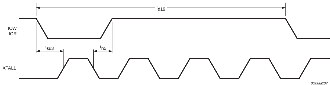
Fig 15. Alternate read/write strobe timing.
