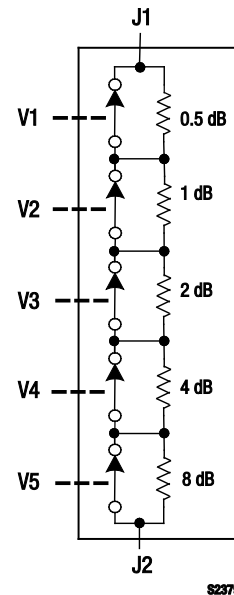
Figure 1. SKY12322-86LF Block Diagram
