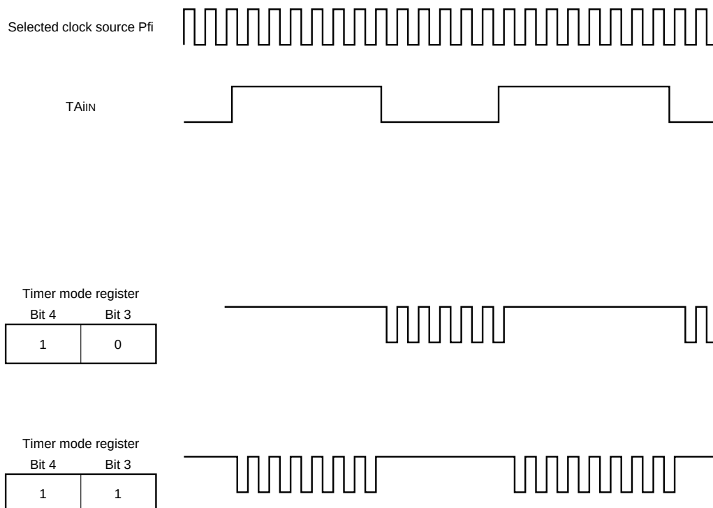
Fig. 20 Count waveform when gate function is available
