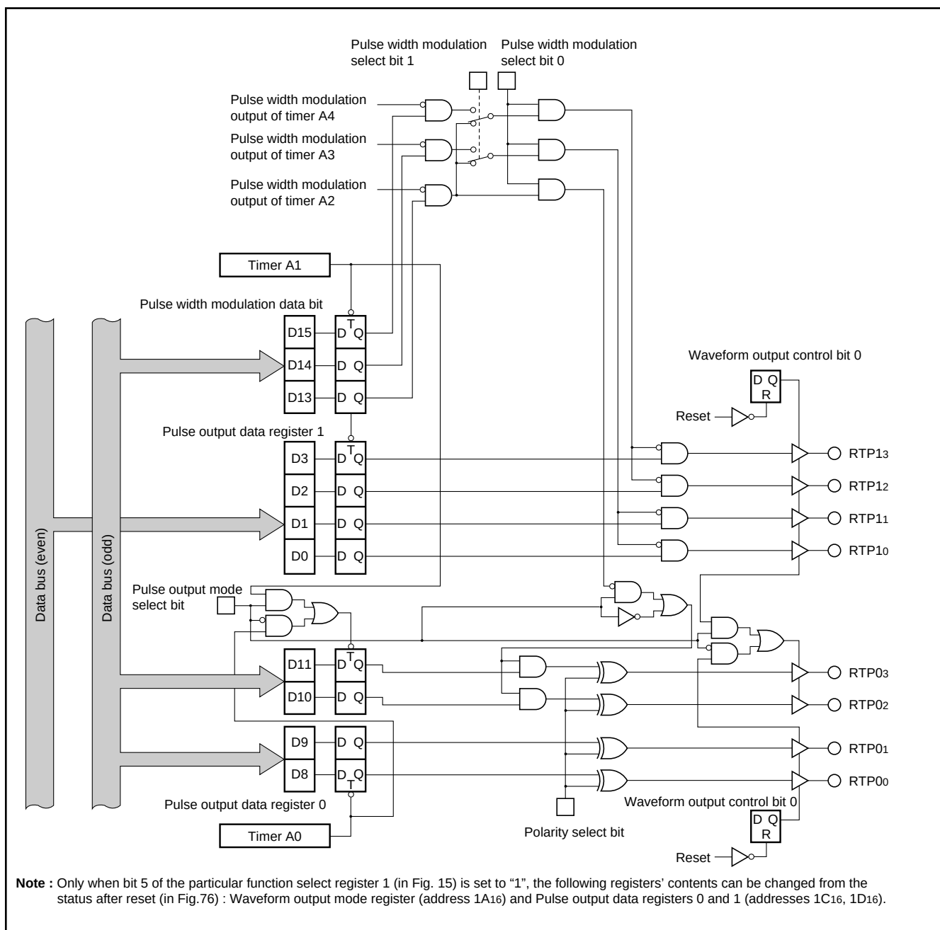
Fig. 48 Pulse output port mode block diagram
