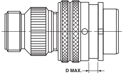
REAR MOUNTING DATA MAXIMUM PANEL THICKNESS
