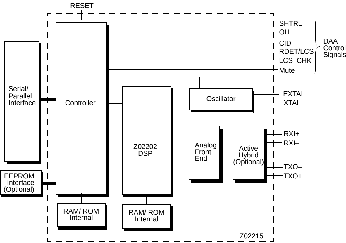
Figure 1. Z02215 Block Diagram
