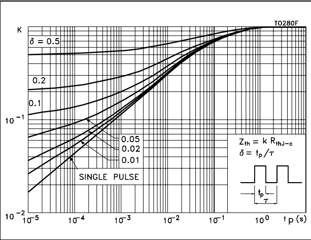
Figure 14. Thermal impedance for TO-220 and D 2 PAK
