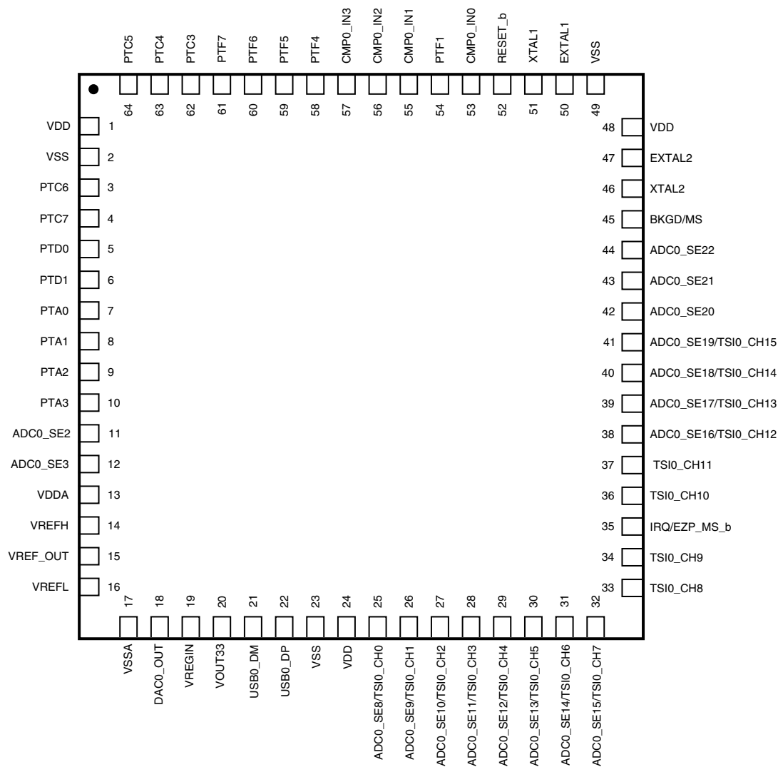
Figure 20. 64-pin LQFP
