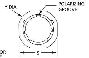
RECEPTACLE ASSEMBLY
