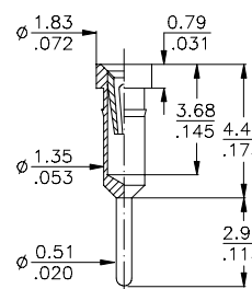
001 Standard terminal
